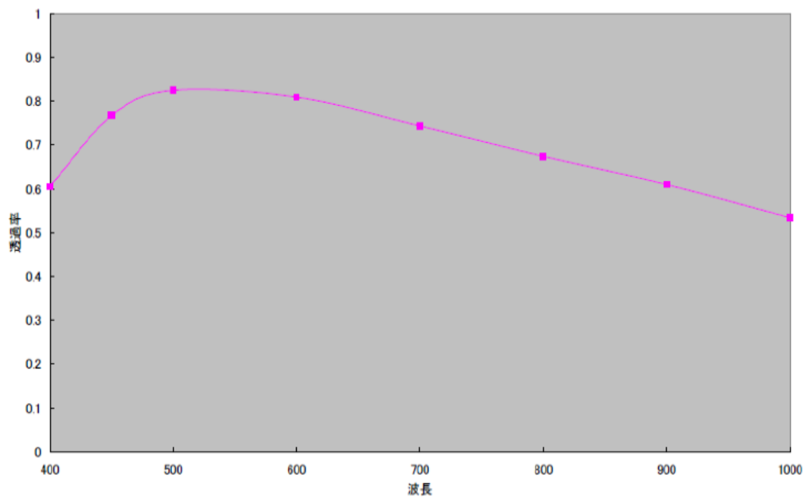
LMVZ9020A-IR Transmission Chart
