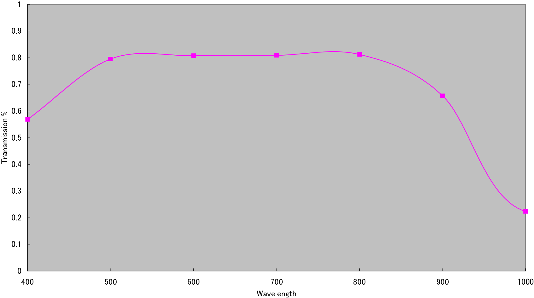
LMZ750 Transmission ( Broad Band Coating )
