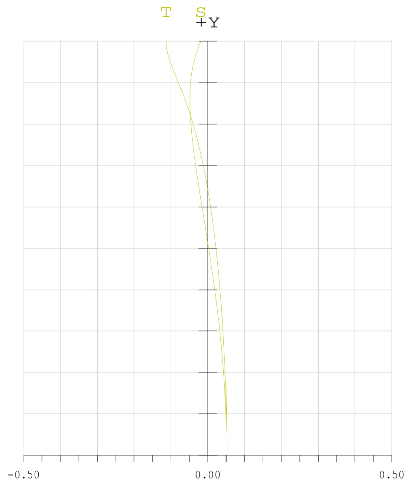
Field Curvature
