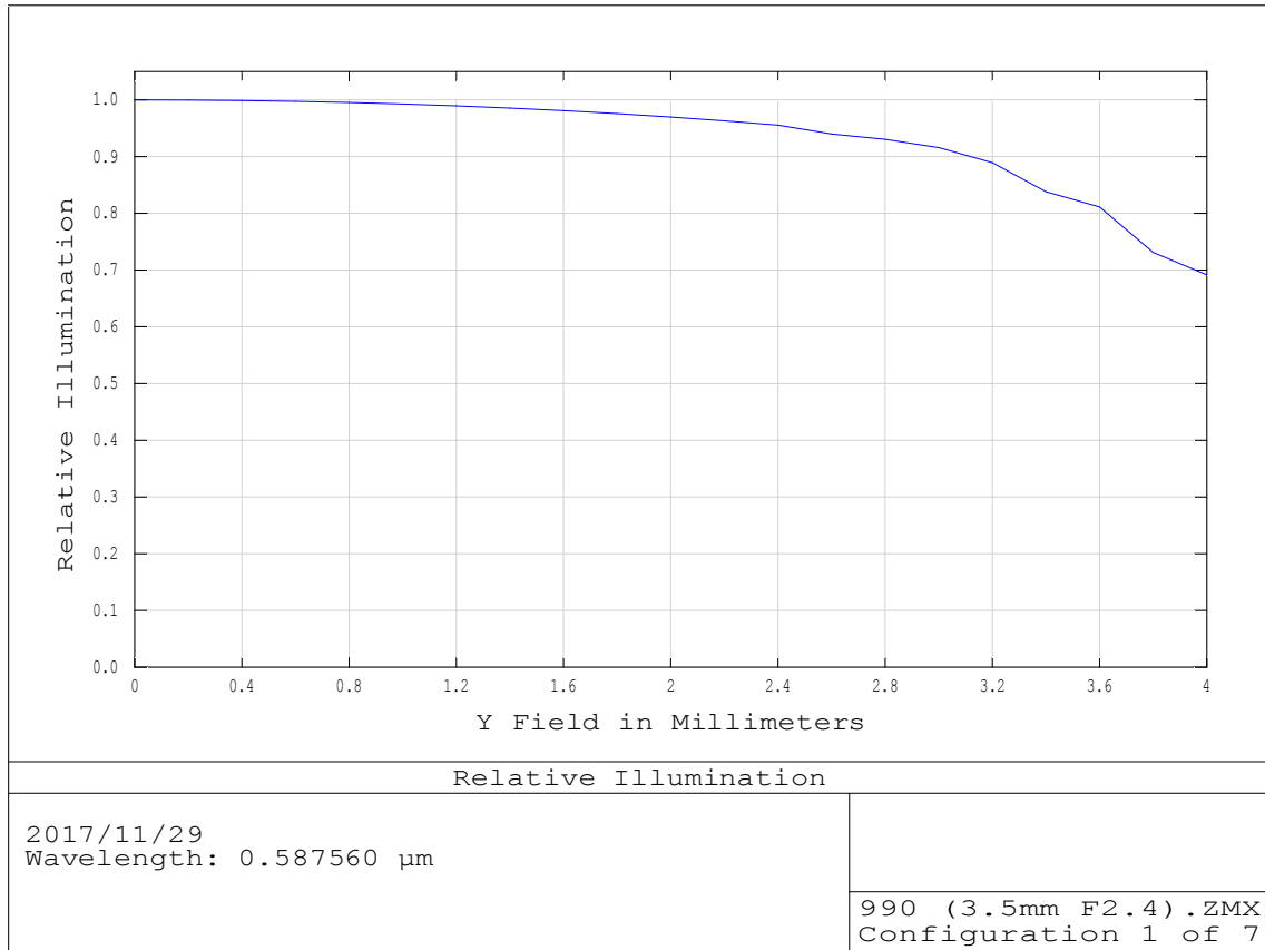
Relative illumination F2.4
