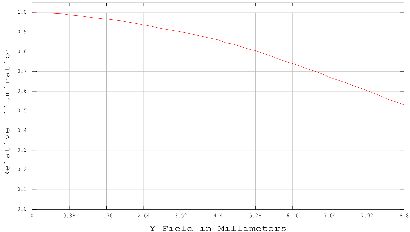
Relative Illumination
