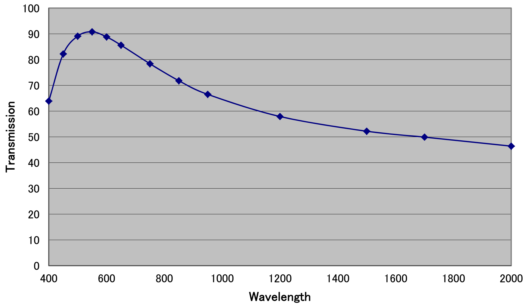
LM5NF Transmission
