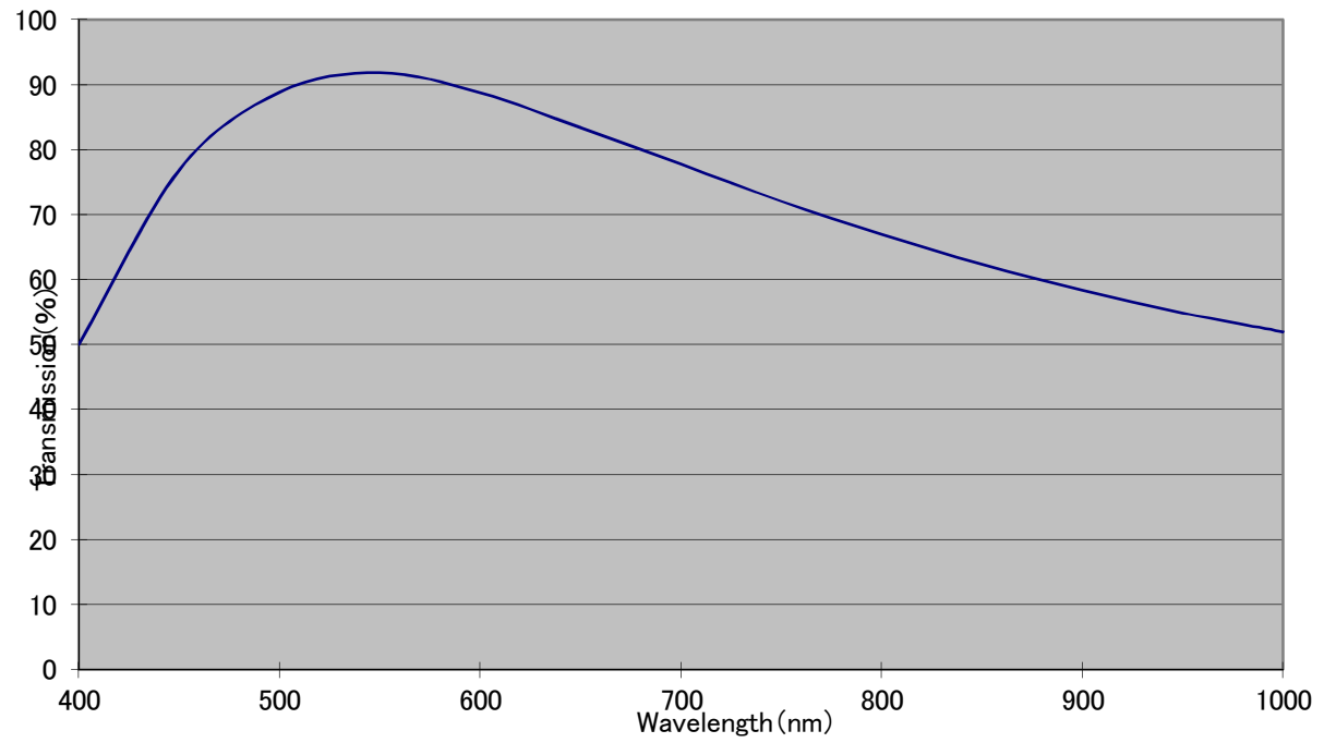
LM6NCM Transmission
