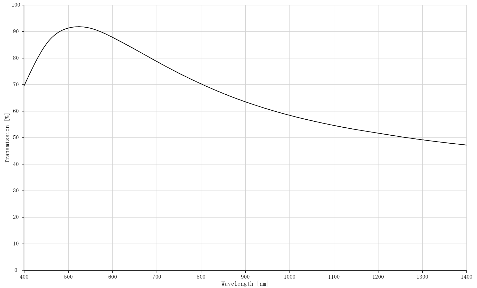
LM8JC5MC-WP Transmission
